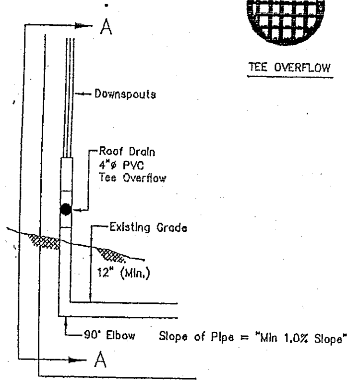
TYPICAL ROOF DRAIN OVERFLOW
